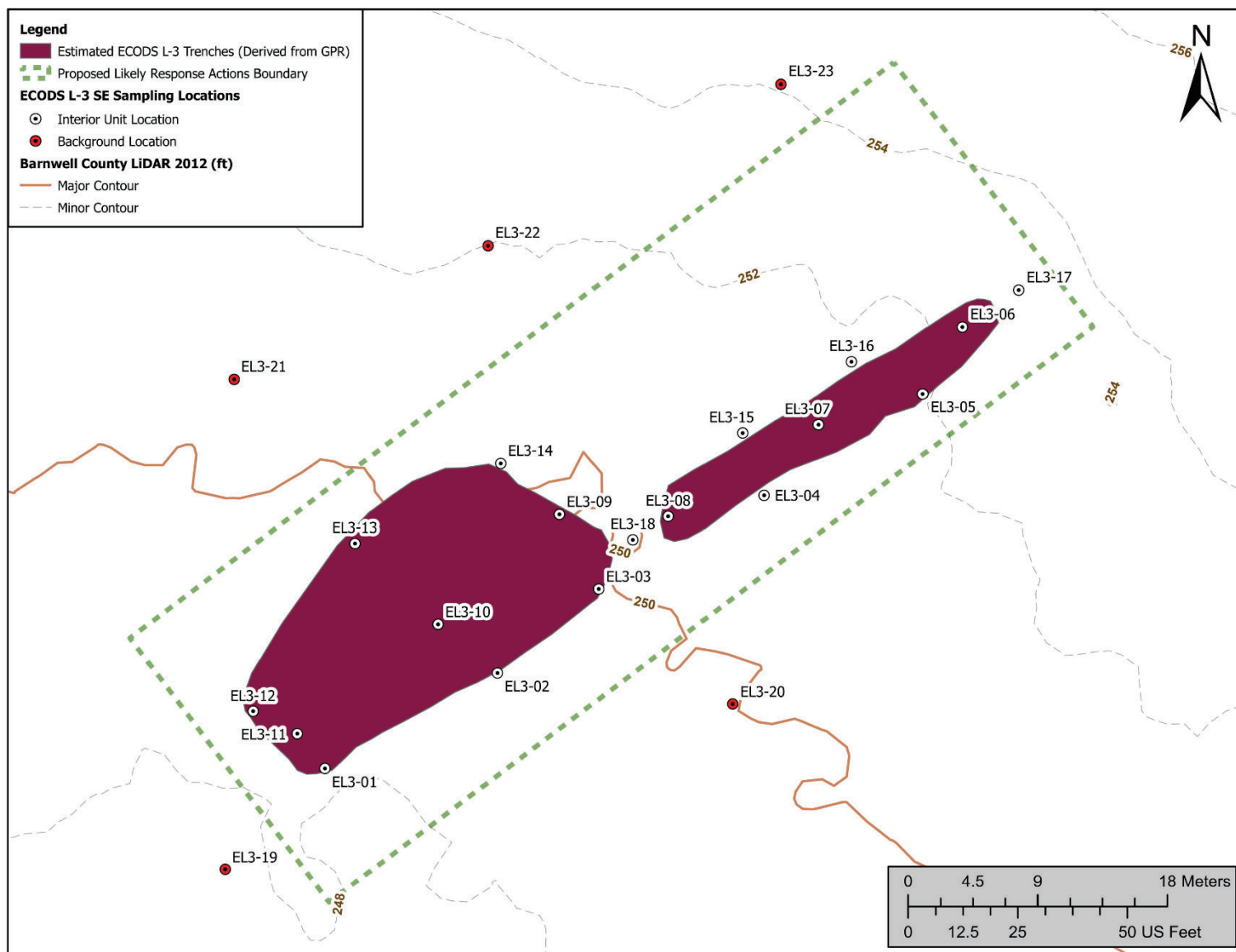
Figure 4. ECODS L-3 Subunit and Site Evaluation Sampling Locations
