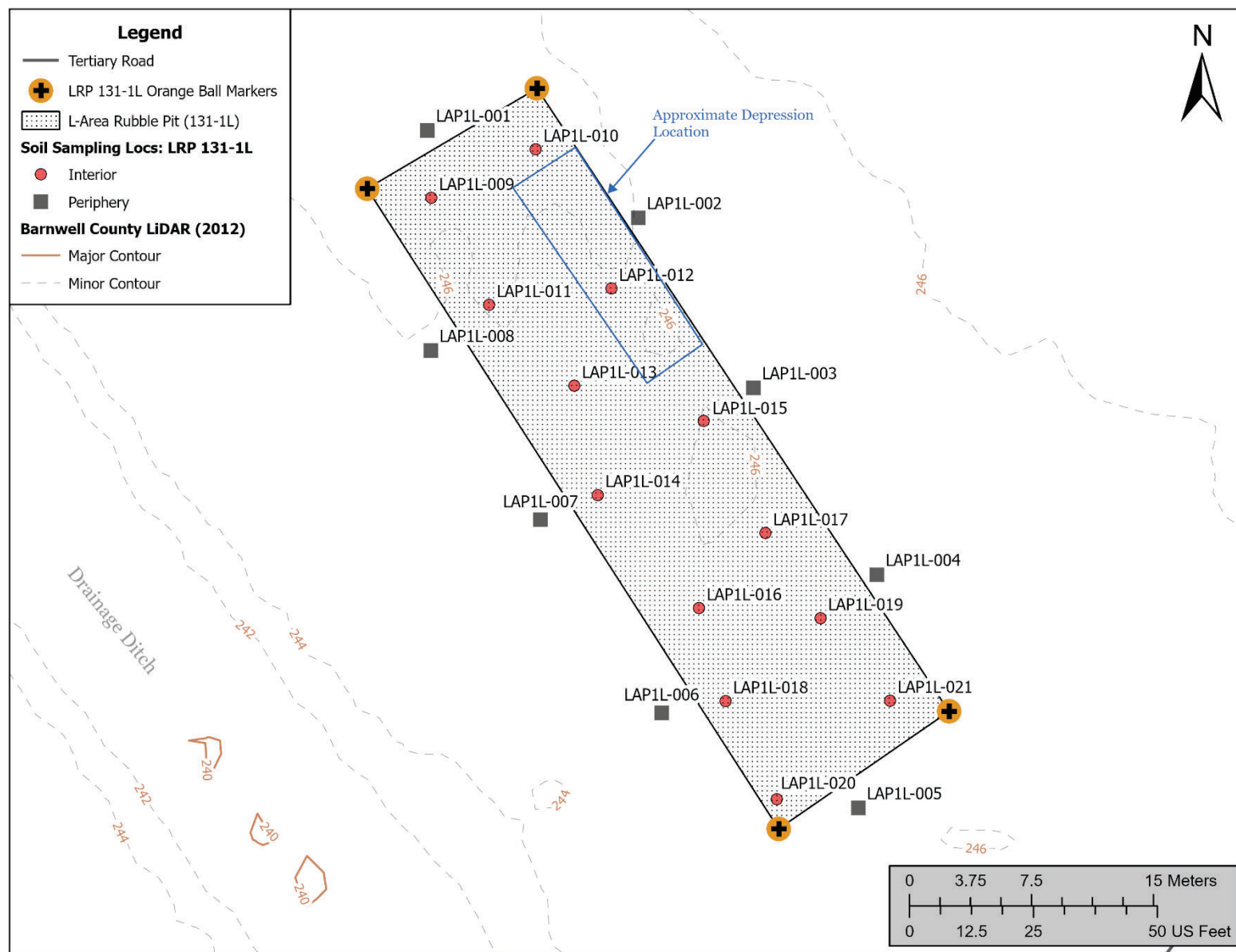
Figure 5. L-Area Rubble Pit 131-1L Subunit and RFI/RI Work Plan Sampling Locations
