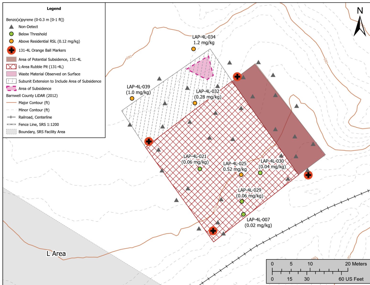
Figure 10. Benzo(a)pyrene Data for Surface Soil Media (0 to 0.3 m [0 to 1 ft]) at the LRP 131-4L Subunit
