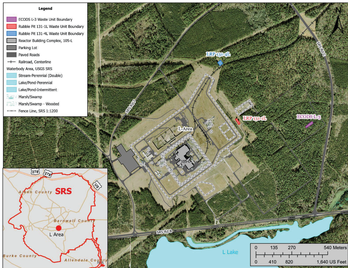
Figure 3. Location of the ECODS L-3, LRP 131-1L, and LRP 131-4L OU within the Savannah River Site
