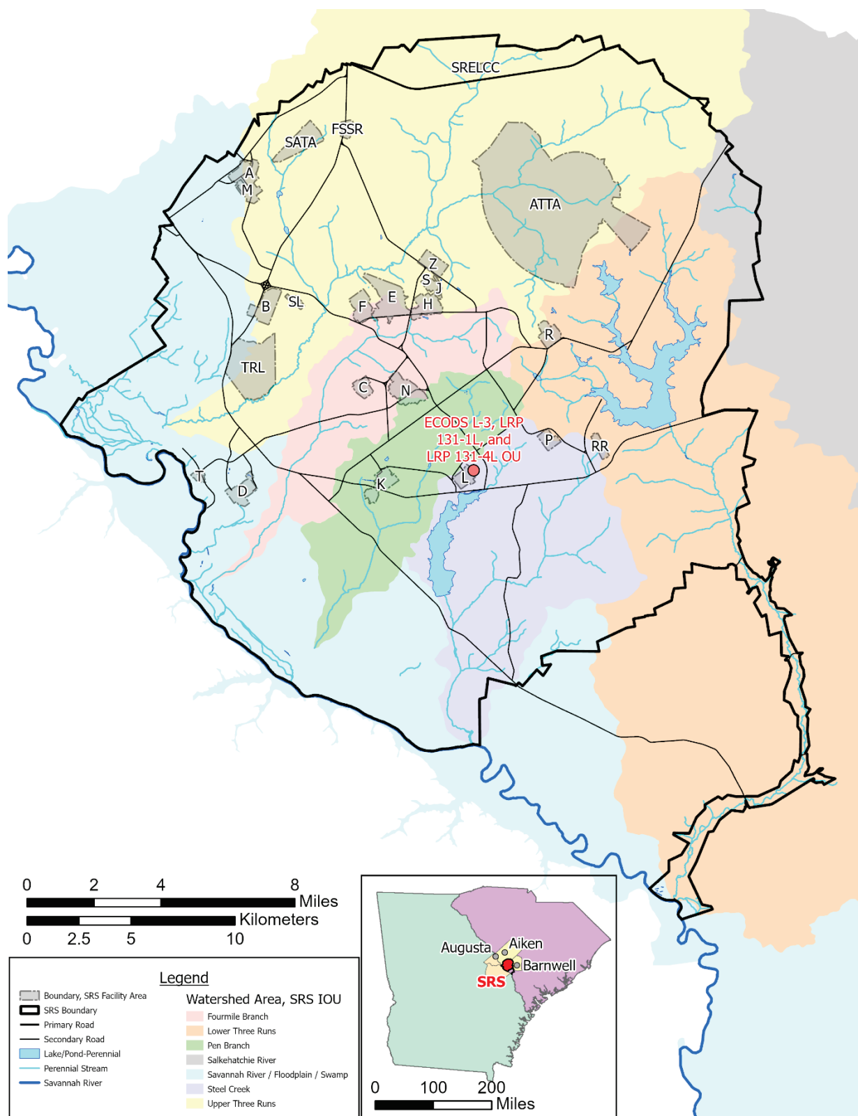
Figure 2. Location of the ECODS L-3, LRP 131-1L, and LRP 131-4L OU at the Savannah River Site
