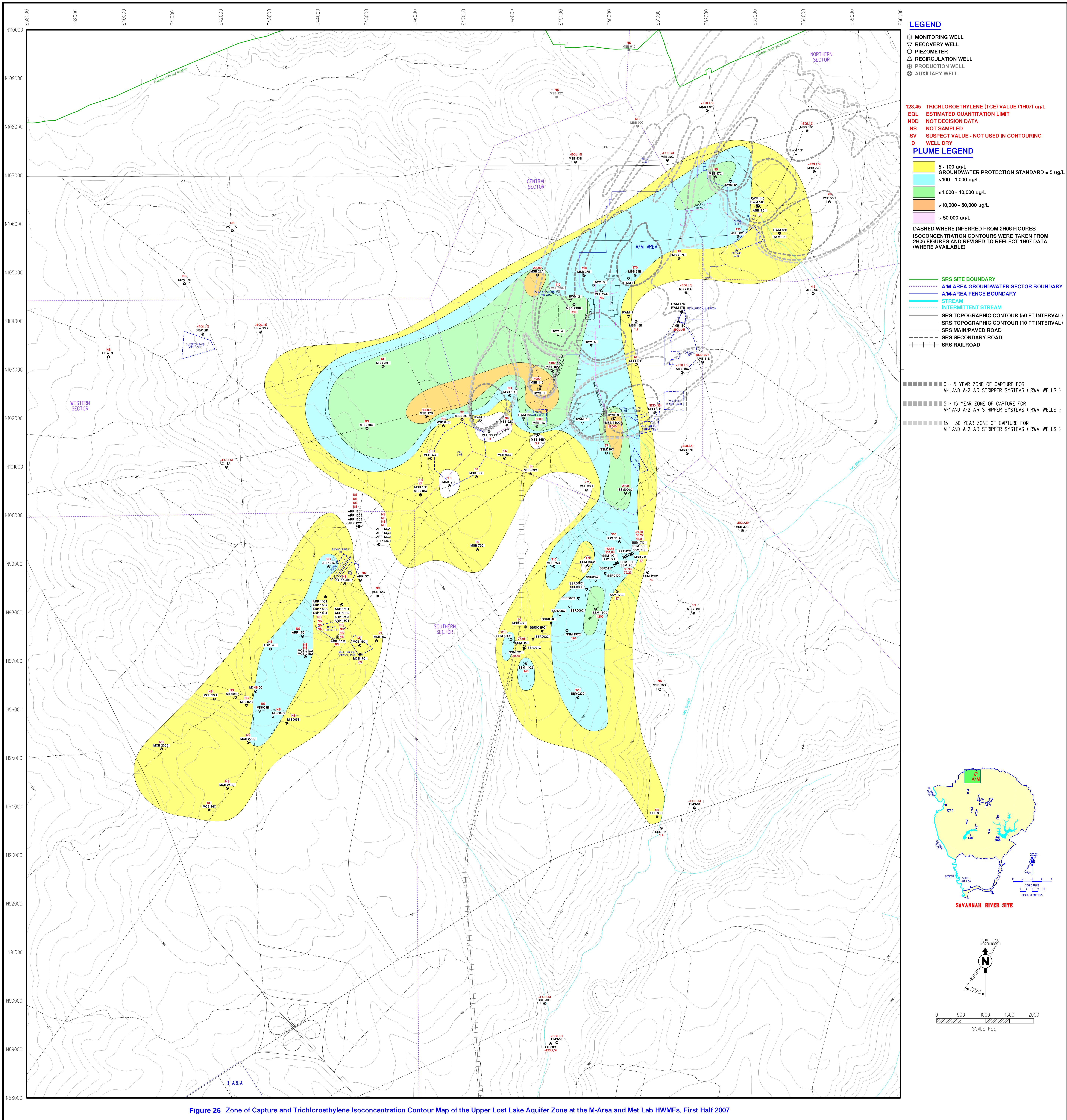
Figure 26 Zone of Capture and Trichloroethylene Isoconcentration Contour Map of the Upper Lost Lake Aquifer Zone at the M-Area and Met Lab HWMFs, First Half 2007
