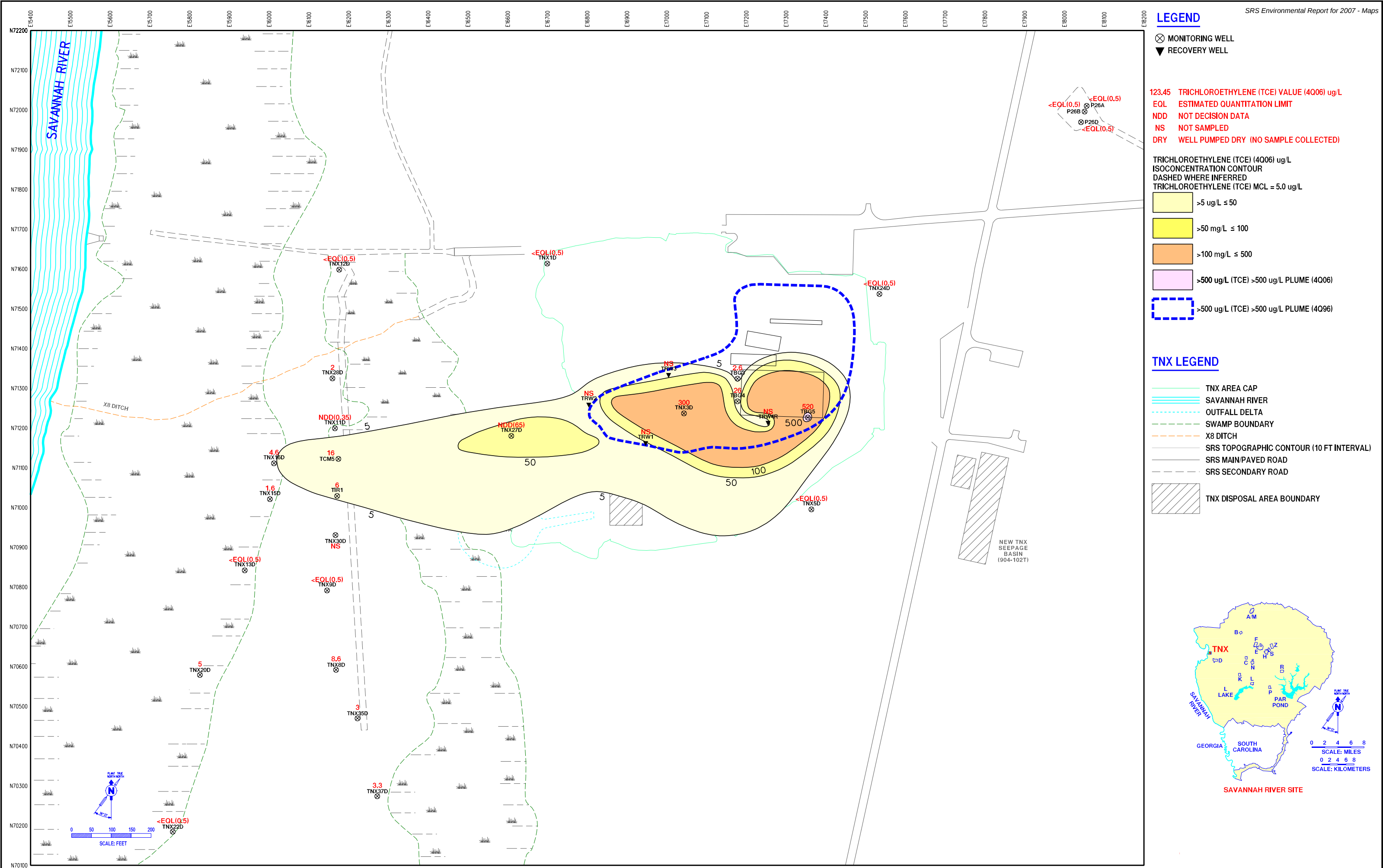
Figure 34 TNX Area Trichloroethylene (TCE) Concentration in Groundwater, 4Q06 with >500 ug/L TCE Plume from 4Q96 Superimposed
